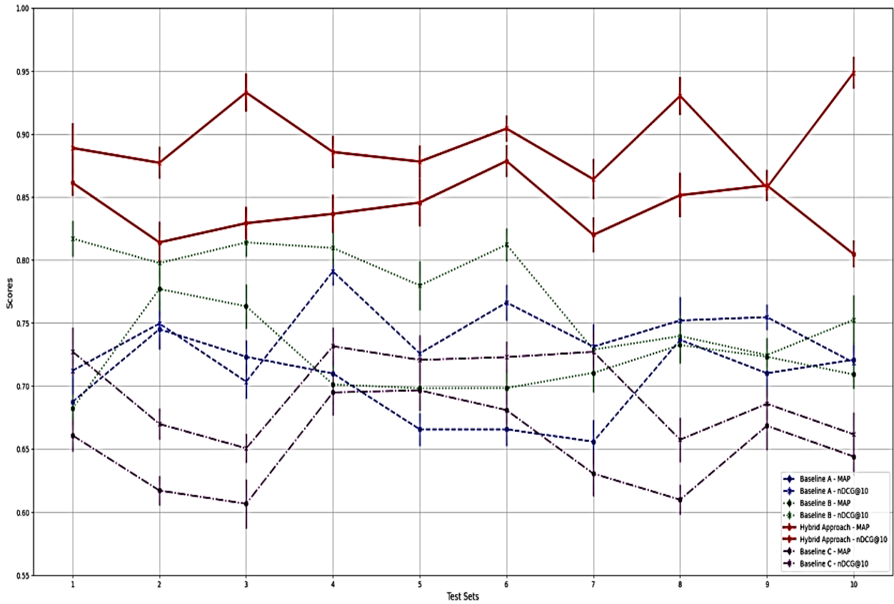
Figure 4: Performance comparison of personalized search methods
