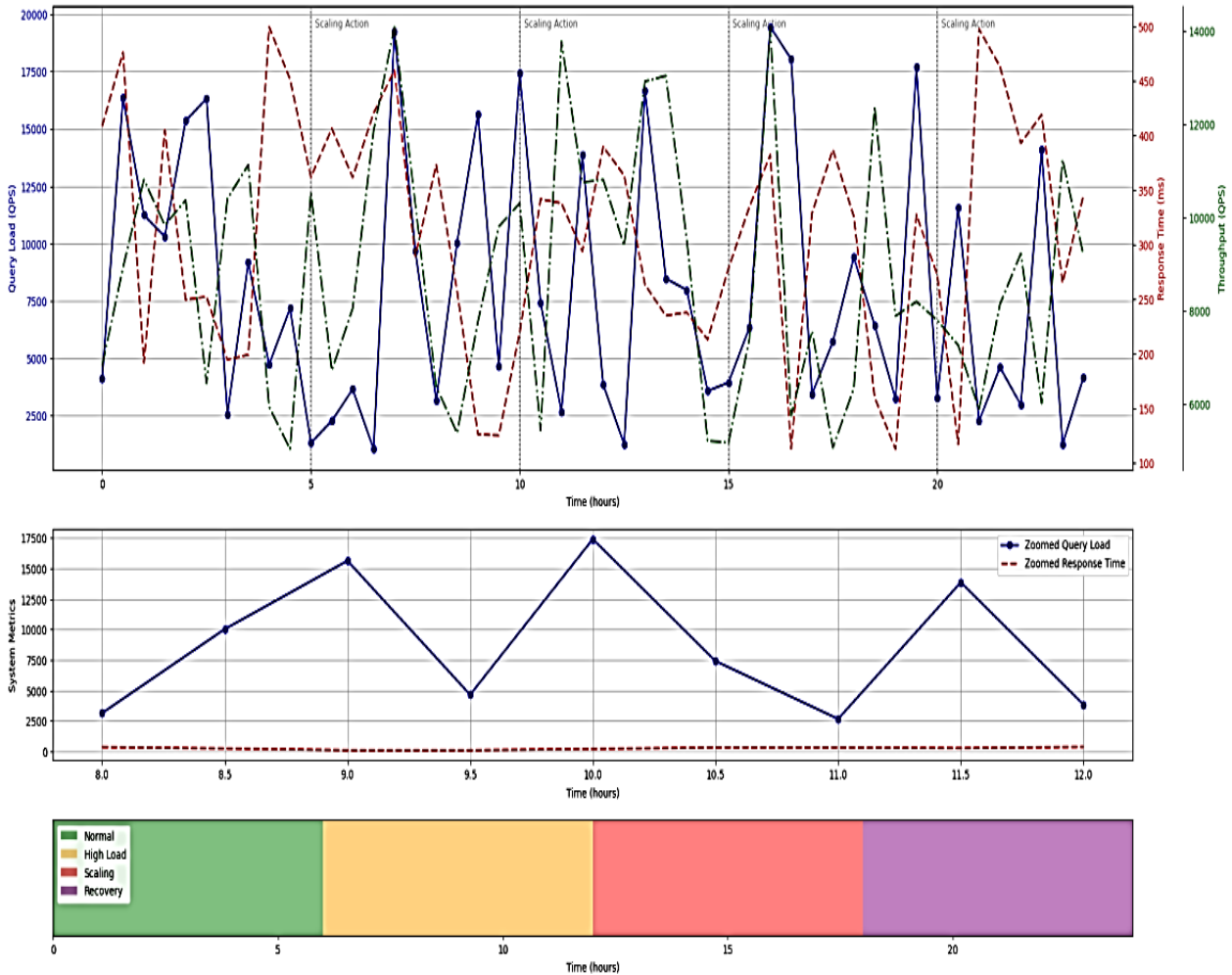
Figure 6: System adaptation to dynamic workloads
