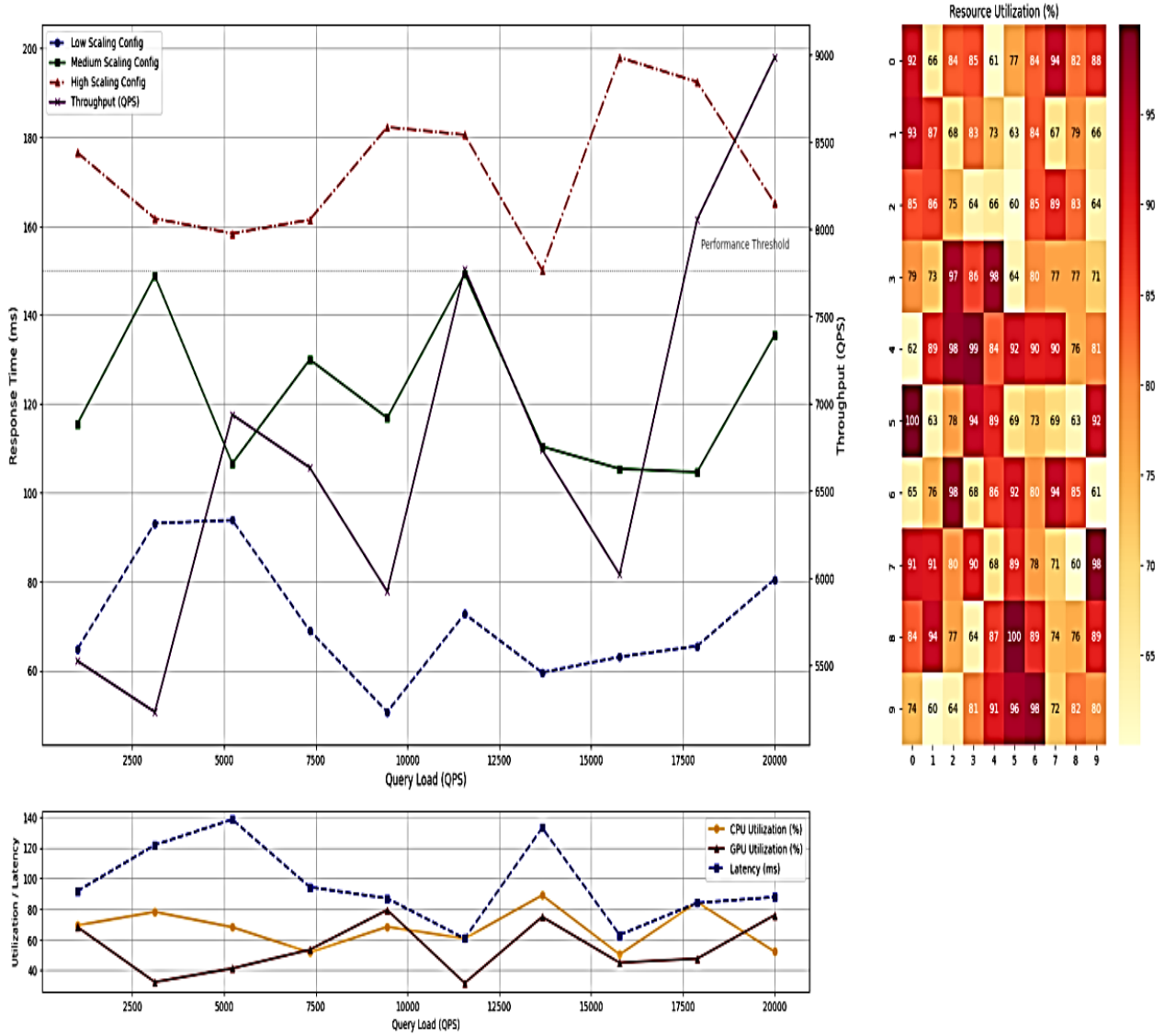
Figure 5: Scalability analysis of the proposed hybrid approach
