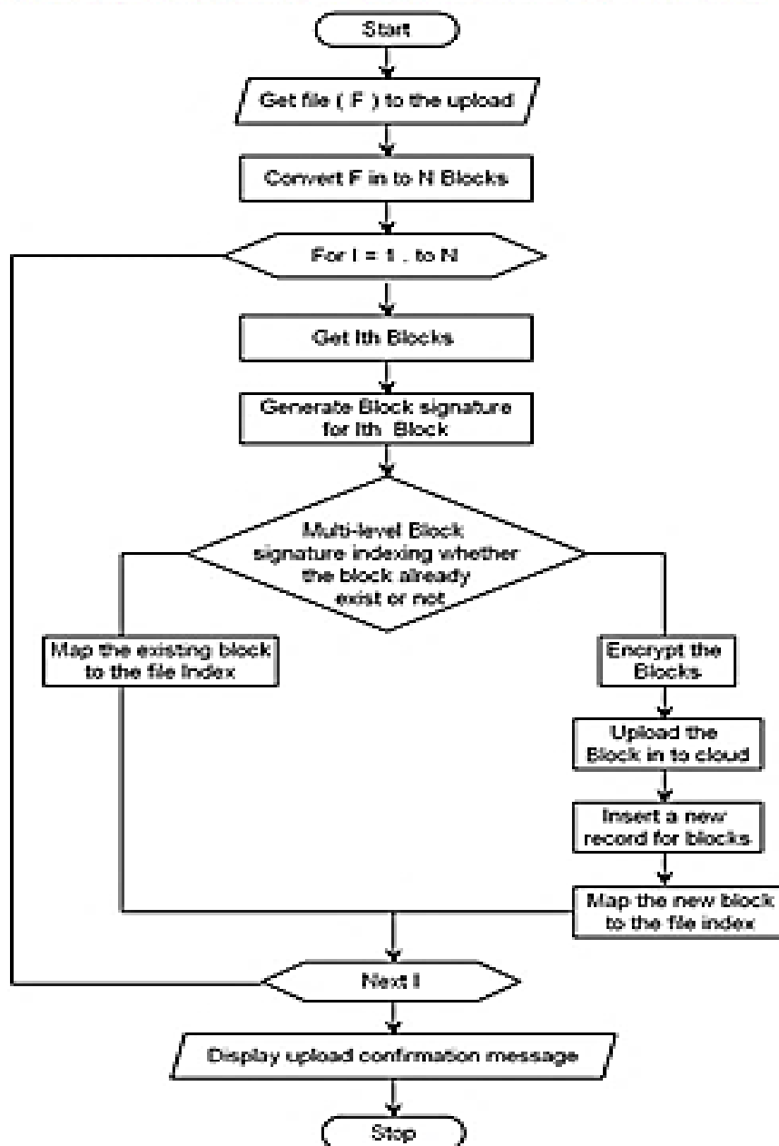
Figure 2: Flow Chart for Upload Process
