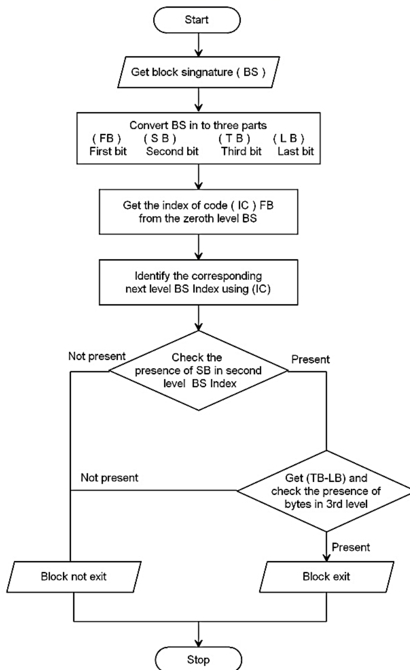
Figure 3: Flow Chart for Multi-Level Block Signature
